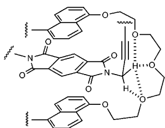
Figure 2. C–H···O contacts in the solid-state structure of 3 .
