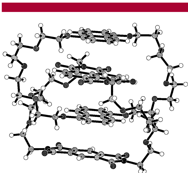
Figure 3. Solid-state structure of [2]catenane 13 .
