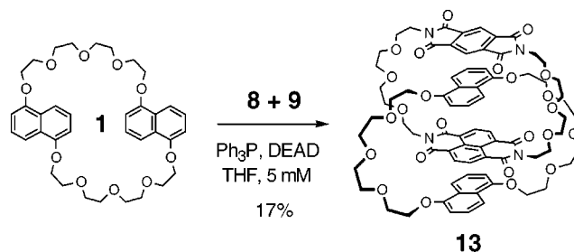
Scheme 3. A [2]Catenane via Mitsunobu Alkylation
