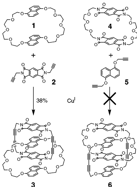
Figure 1. Successful and unsuccessful [2]catenane syntheses.
